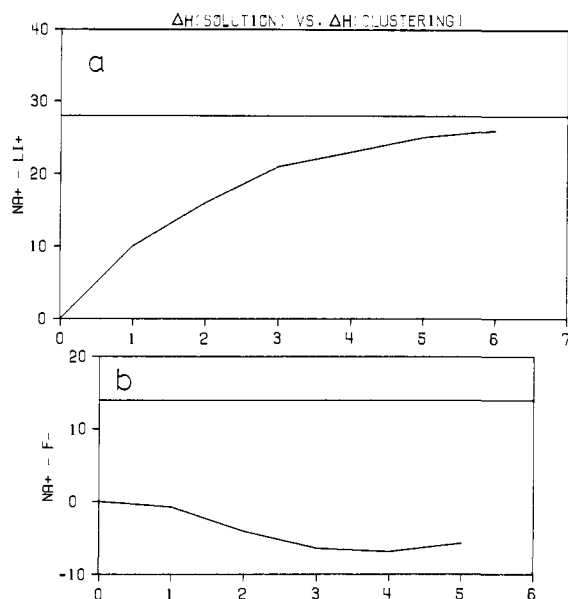
Figure 1. Differences in gas-phase clustering enthalpies (kcal/mol) as a function of cluster size for (a) Na + and Li + and (b) Na + and F - . The differences in the total heats of solution are shown as horizontal lines.
